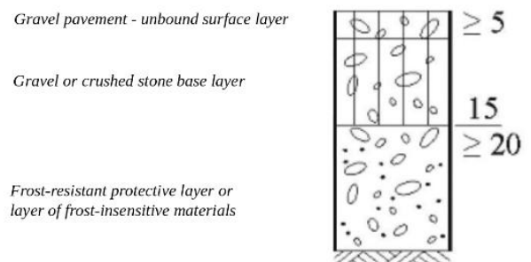
Fig. 5.14.1 Diagram of gravel road restoration.
