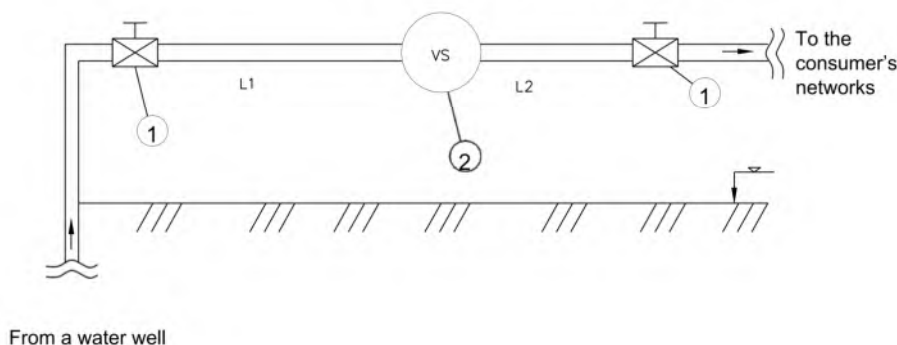
DIAGRAM OF THE WATER METERING STATION
