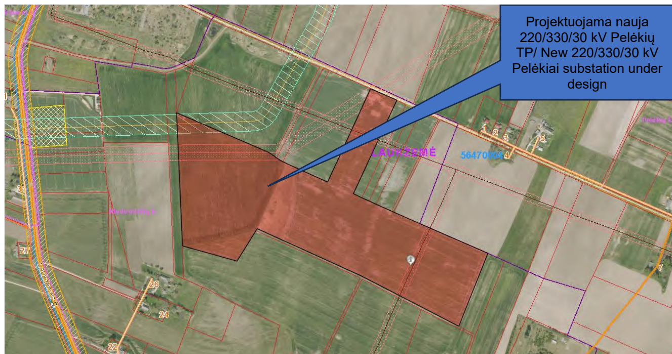
4 pav. Planuojamo statyti statinio schema teritorijų, kuriose taikomos SŽNS, kontekste / Fig. 4. Schematic diagram of the planned structure in the context of areas subject to the Special Protection Zone
